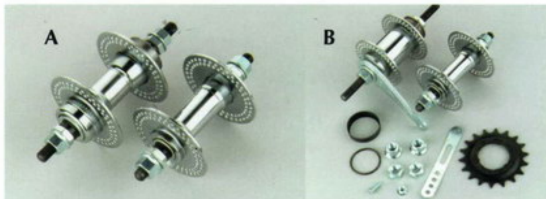
A 140H OR 144H NORMAL HUB SET
